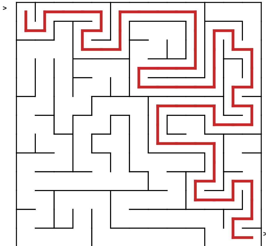
Maze 1 - solution
