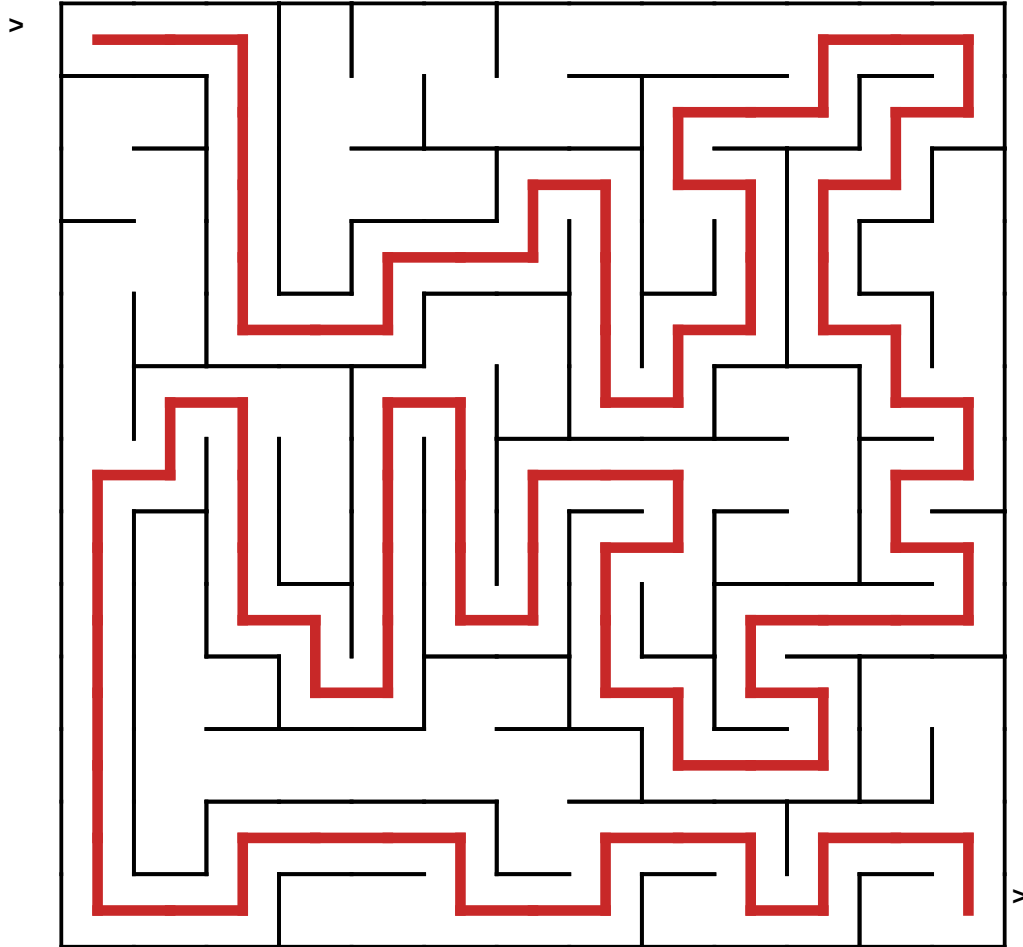
Maze 5 - solution
