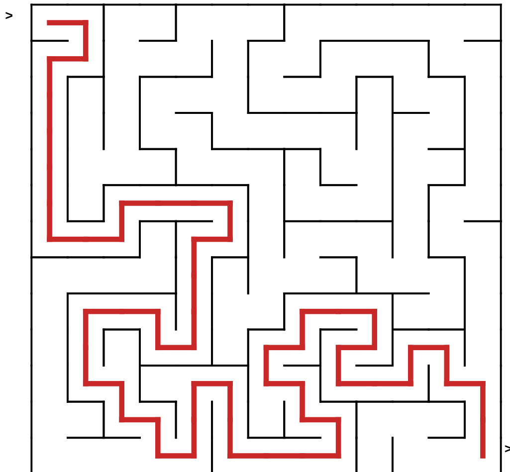
Maze 7 - solution
